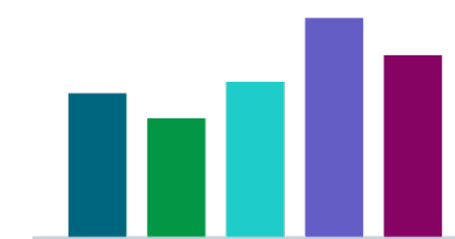
Bar Chart
