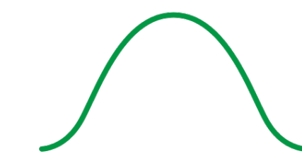
Line histogram
