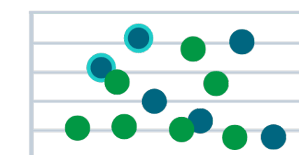
Scatter plot
