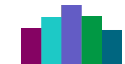
Bar histogram
